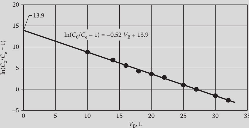
FIGURE 15.32 Linear plot of \ln(C_0/C_e - 1) versus V_B (Example 15.47).
