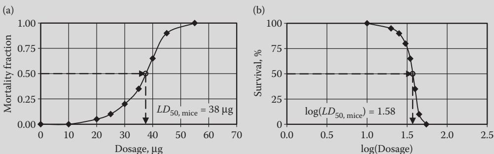
FIGURE 12.3 Dose–response curves for determining pesticide toxicity to mice: (a) arithmetic plot and (b) semi-log plot (Example 12.3).
