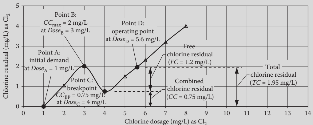
FIGURE 11.11 Plot of chlorine residual curve (Example 11.27).
