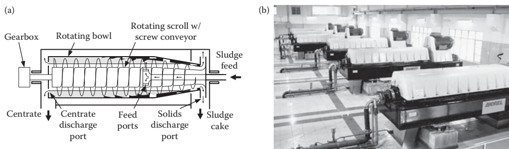
FIGURE 13.25 Decanter solid-bowl centrifugal dewatering: (a) components of a typical centrifuge and (b) general arrangement of centrifuges for dewatering (Courtesy Andritz (USA) Inc.).
