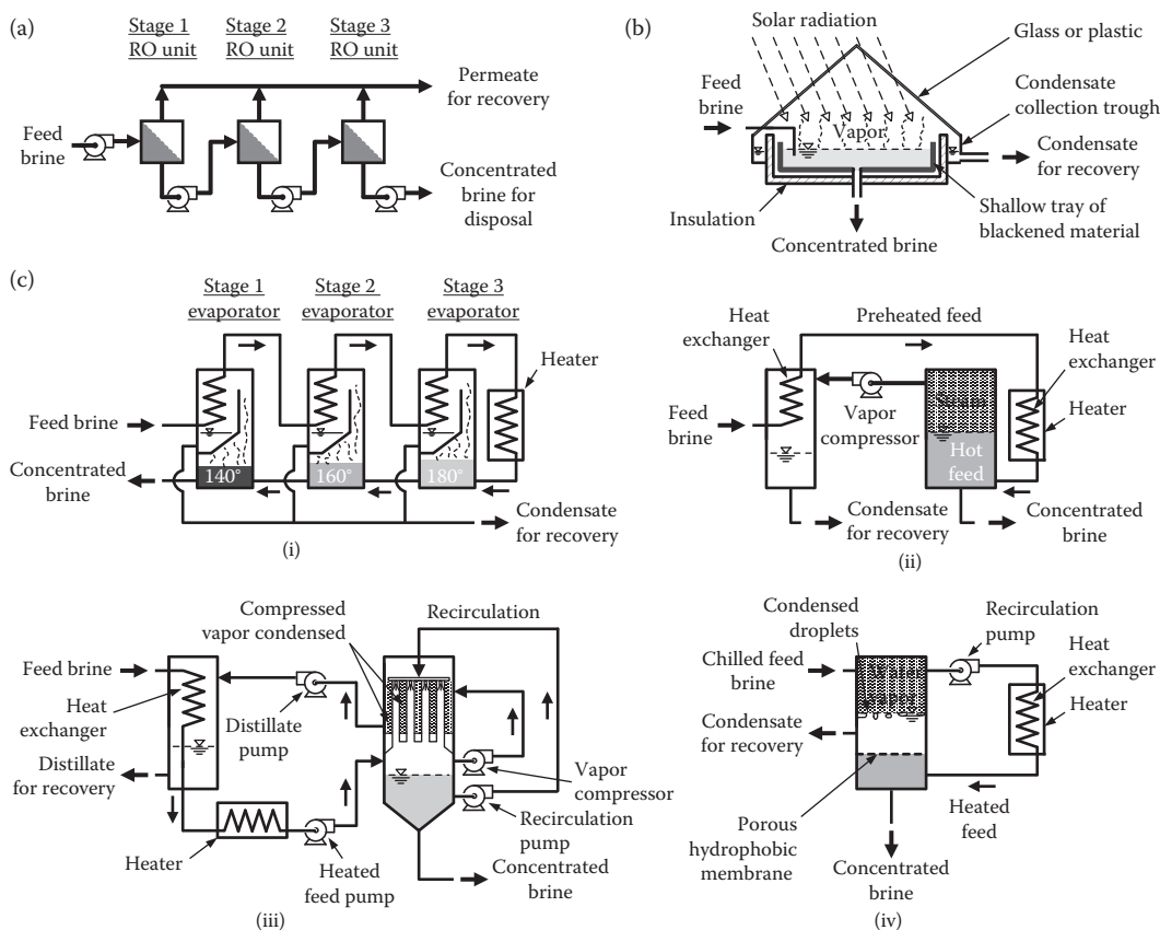
FIGURE 15.41 Concentration of brine: (a) multiple-stage RO; (b) solar evaporation; and (c) controlled thermal distillation: (i) multiple-effect distillation, (ii) distillation with vapor compression, (iii) falling-film evaporator, and (iv) membrane distillation.
