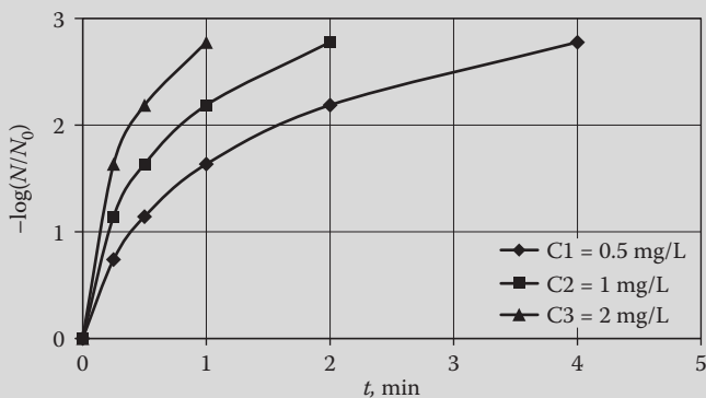
FIGURE 11.7 Plot of -\log(N/N_0) versus t at different C values using Selleck equation (Example 11.13).
