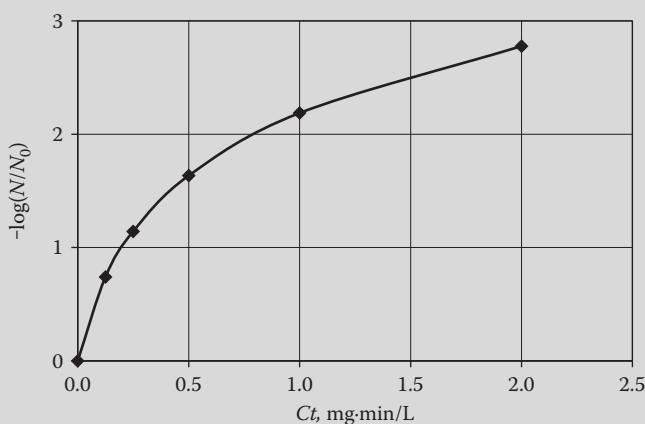
FIGURE 11.6 Plot of -\log(N/N_0) versus Ct using Selleck equation (Example 11.13).
