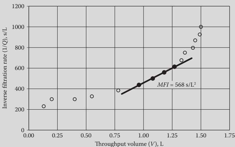
FIGURE 15.38 Plot of inverse flow rate versus throughput volume for determination of MFI (Example 15.57).
