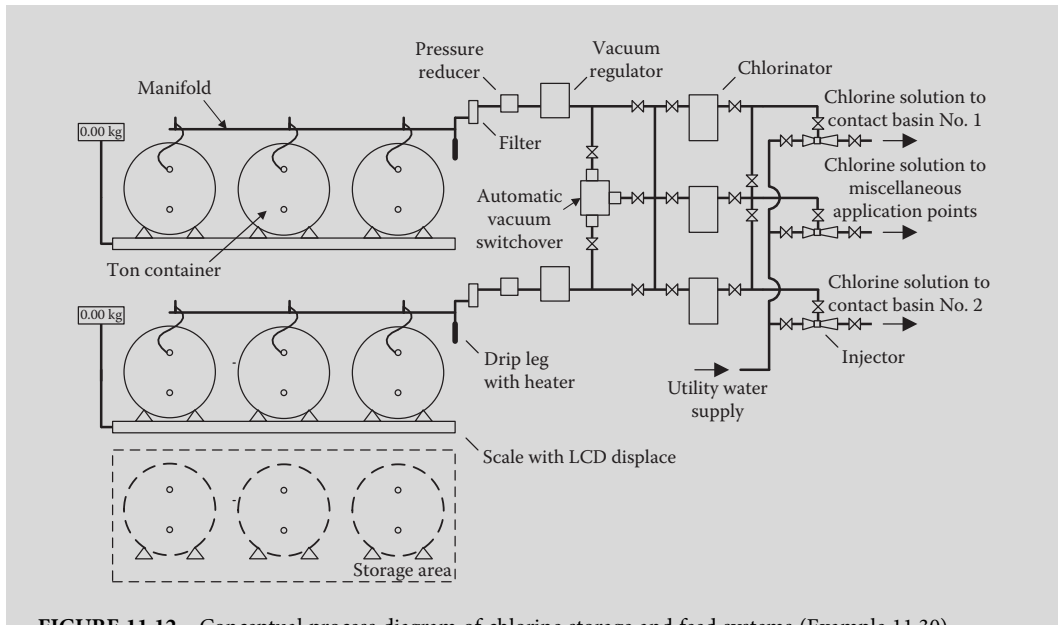
FIGURE 11.12 Conceptual process diagram of chlorine storage and feed systems (Example 11.30).
