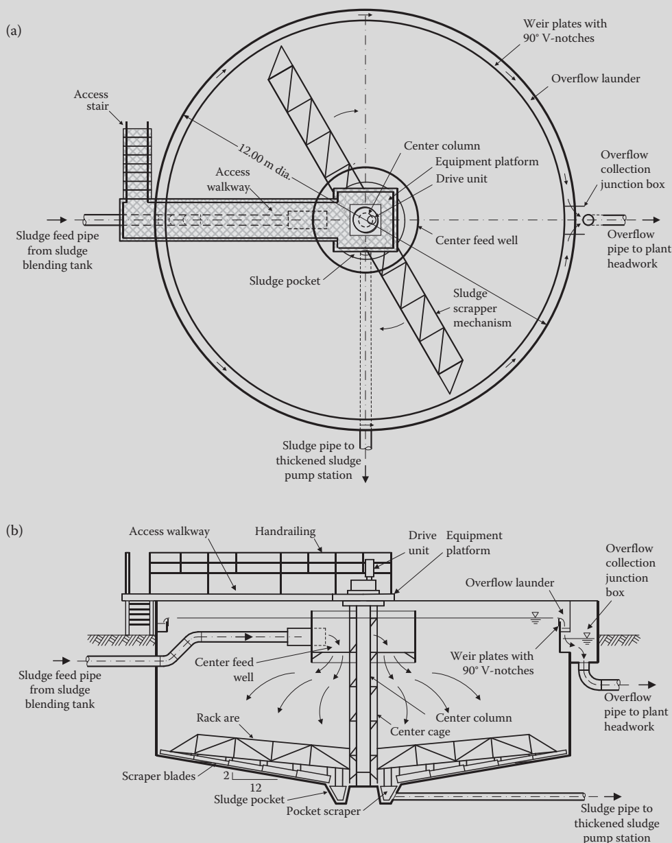
FIGURE 13.3 Design details of gravity thickener: (a) plan view (Example 13.12). (b) conceptual sectional view (Example 13.12).
