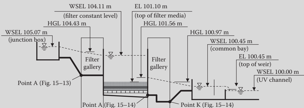
FIGURE 15.15 Hydraulic profile through the tertiary filter system (Example 15.25).
