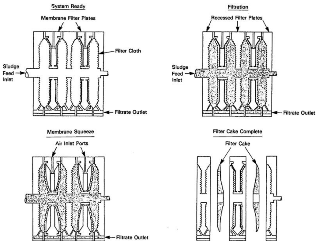
FIGURE 13.26 Recessed plate filter press dewatering cycle. (Adapted in part from Reference 74; Courtesy U.S. EPA.)
