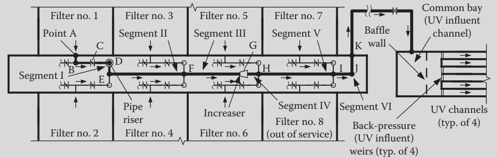
FIGURE 15.14 Details of filter effluent piping, including combined filter effluent conduit, and common bay with back-pressure weirs (Example 15.24).
