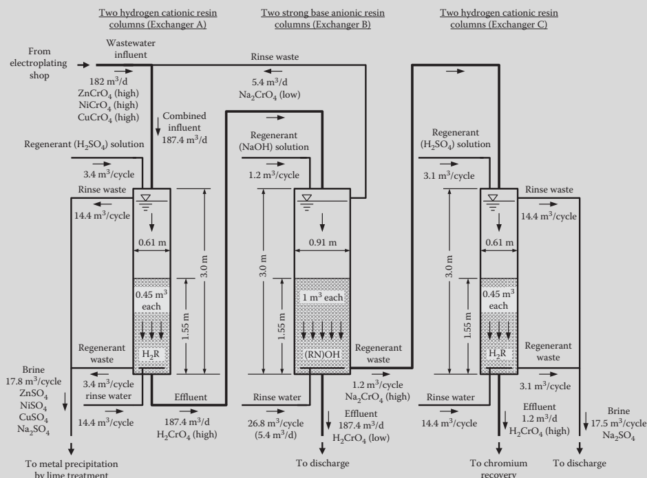
FIGURE 15.33 Process diagram of ion exchange system for metal removal and recovery of chromium (Example 15.48).
