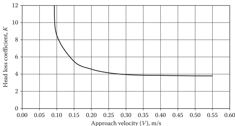
FIGURE 11.29 Head loss coefficient K through two banks arranged in series. (Developed from the information contained in Reference 42.)
