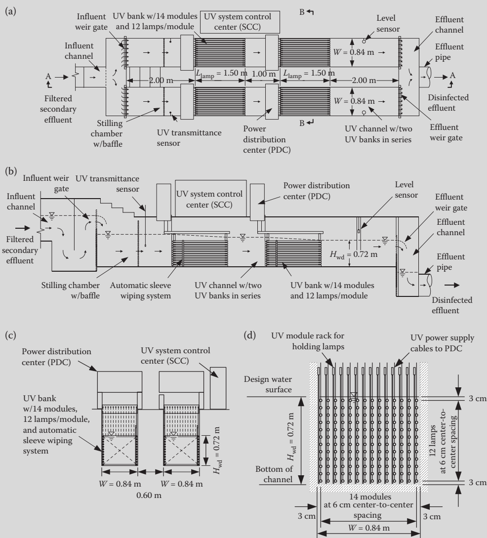
FIGURE 11.31 Design details of the UV disinfection system: (a) plan showing two UV channels in parallel operation, (b) Section AA, (c) Section BB, and (d) arrangement of modules and lamps (Example 11.61).
